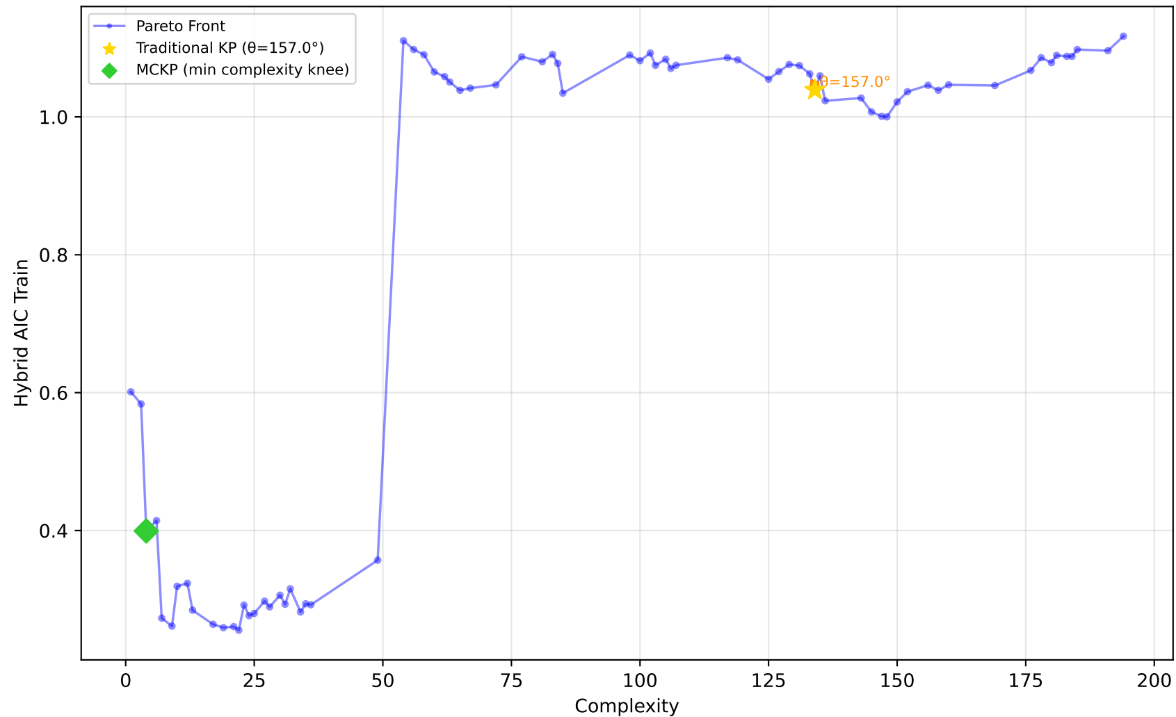
228_elusage - Run 7 - MVP - Hybrid AIC Train \lambda_1=0.00, \lambda_2=0.00, \lambda_3=1.00 | Difficulty: 1.00 | Method: hmr
