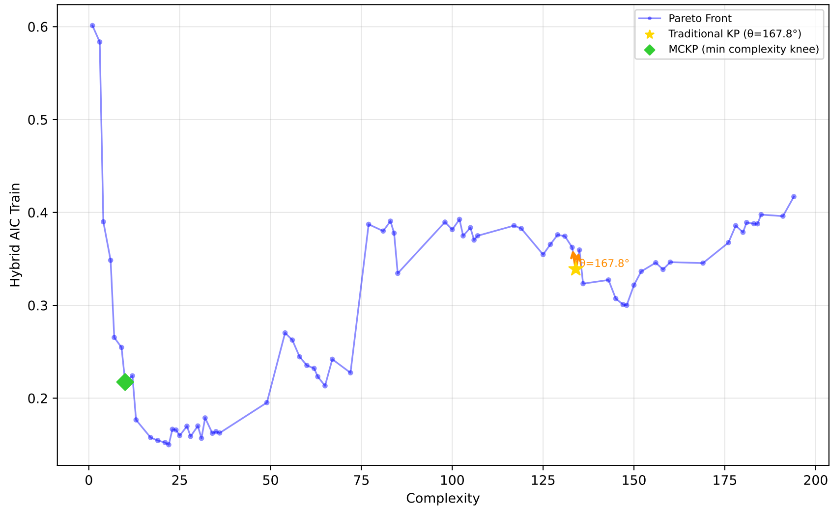
228_elusage - Run 7 - MVP - Hybrid AIC Train \lambda_1=0.00, \lambda_2=0.30, \lambda_3=0.00 | Difficulty: 1.00 | Method: hmr
