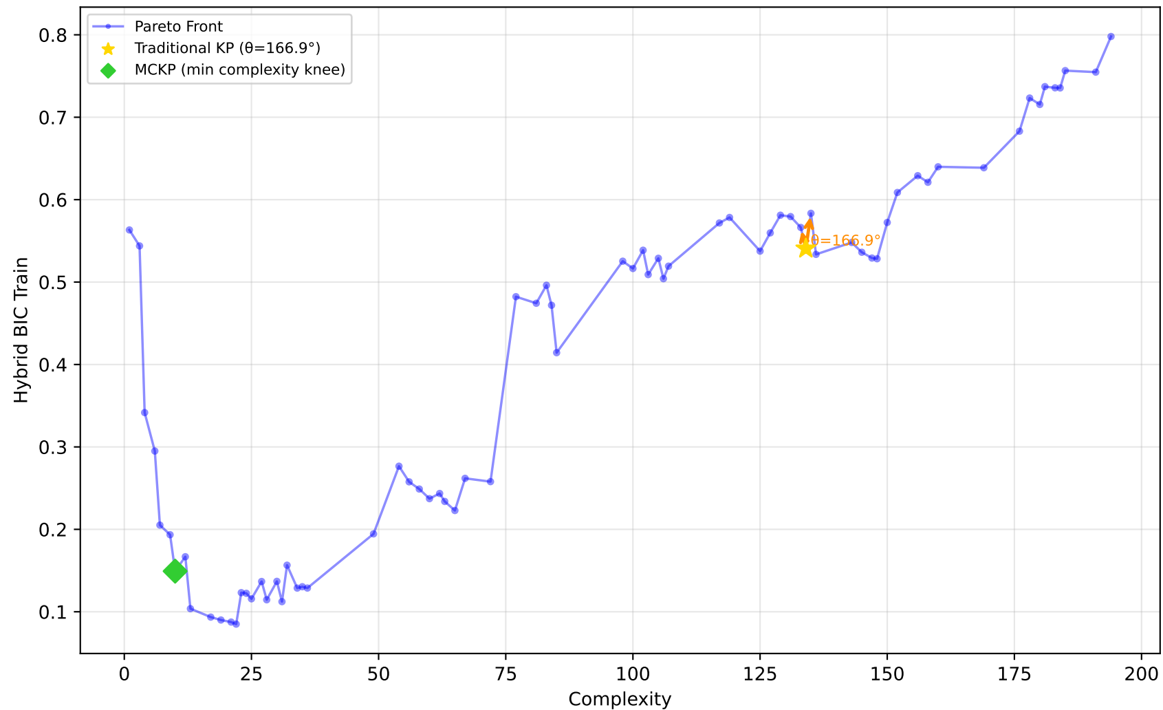
228_elusage - Run 7 - MVP - Hybrid BIC Train \lambda_1=0.00, \lambda_2=0.30, \lambda_3=0.00 | Difficulty: 1.00 | Method: hmr
