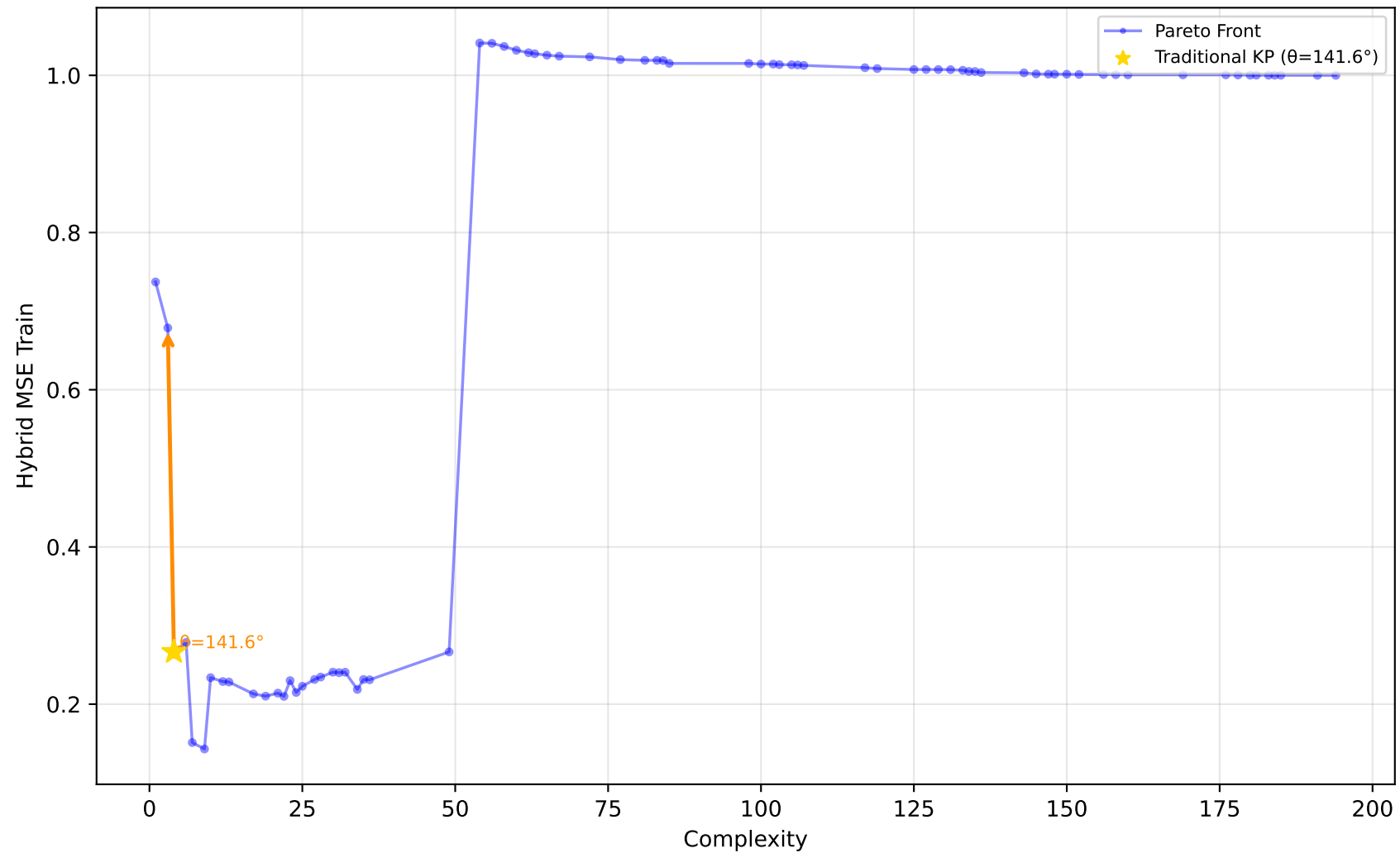
228_elusage - Run 7 - MVP - Hybrid MSE Train \lambda_1=0.00, \lambda_2=0.00, \lambda_3=1.00 | Difficulty: 1.00 | Method: hmr
