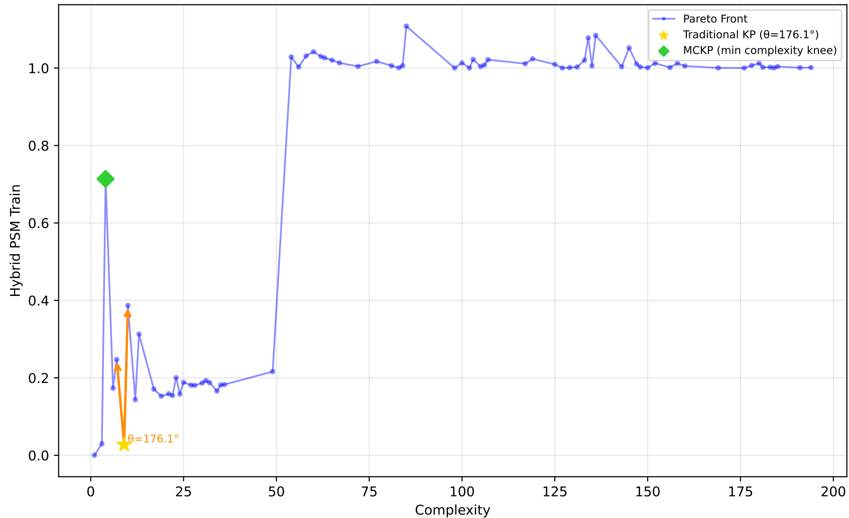
228_elusage - Run 7 - MVP - Hybrid PSM Train \lambda_1=0.00, \lambda_2=0.00, \lambda_3=1.00 | Difficulty: 1.00 | Method: hmr
