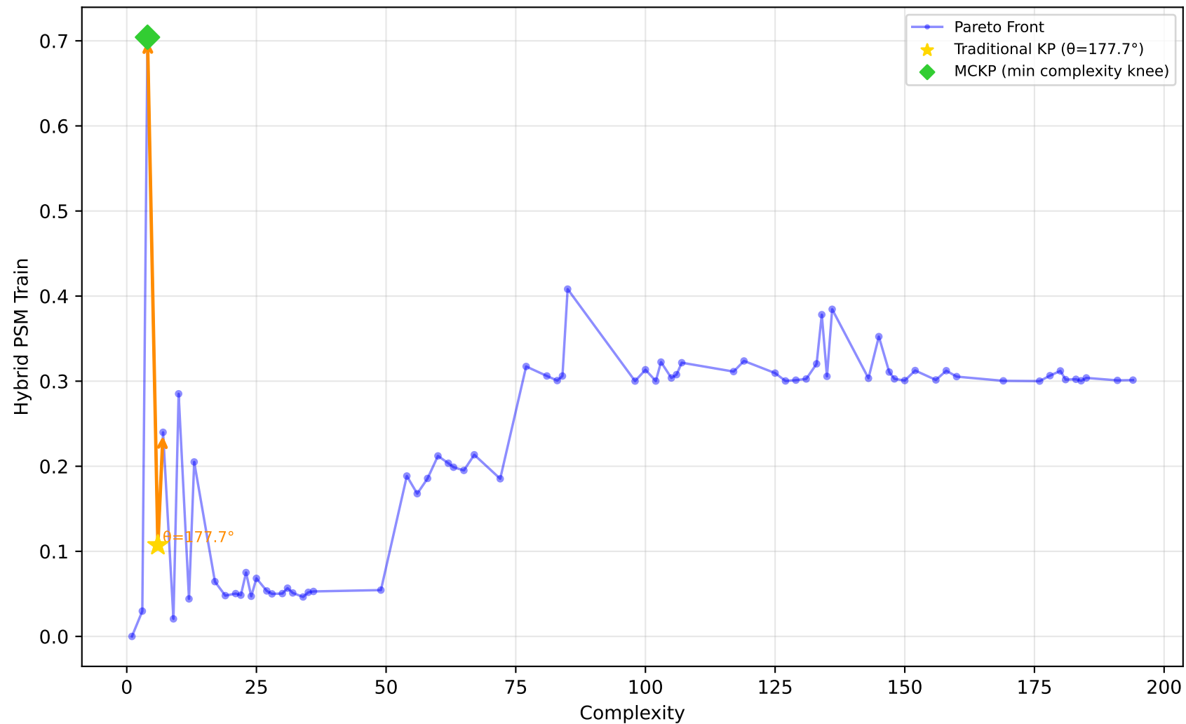
228_elusage - Run 7 - MVP - Hybrid PSM Train \lambda_1=0.00, \lambda_2=0.30, \lambda_3=0.00 | Difficulty: 1.00 | Method: hmr
