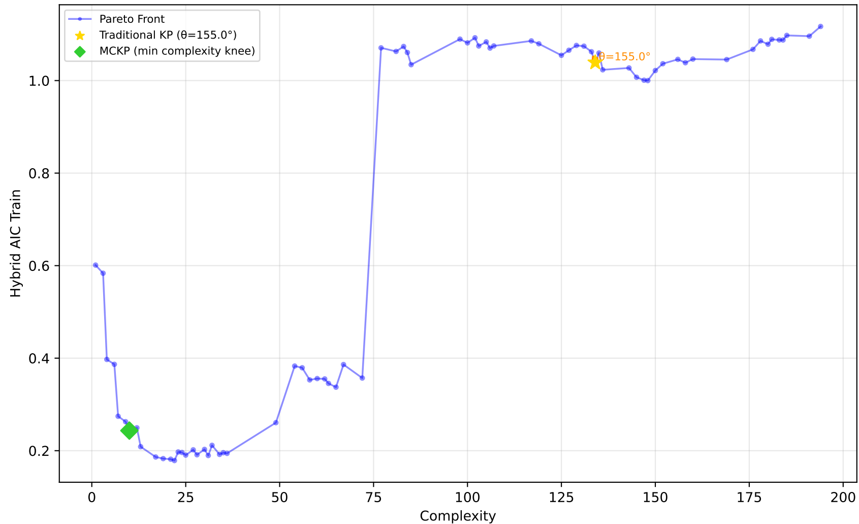
228_elusage - Run 7 - SVP - Hybrid AIC Train \lambda_1=0.00, \lambda_2=1.00, \lambda_3=0.00 | Difficulty: 1.00 | Method: hmr
