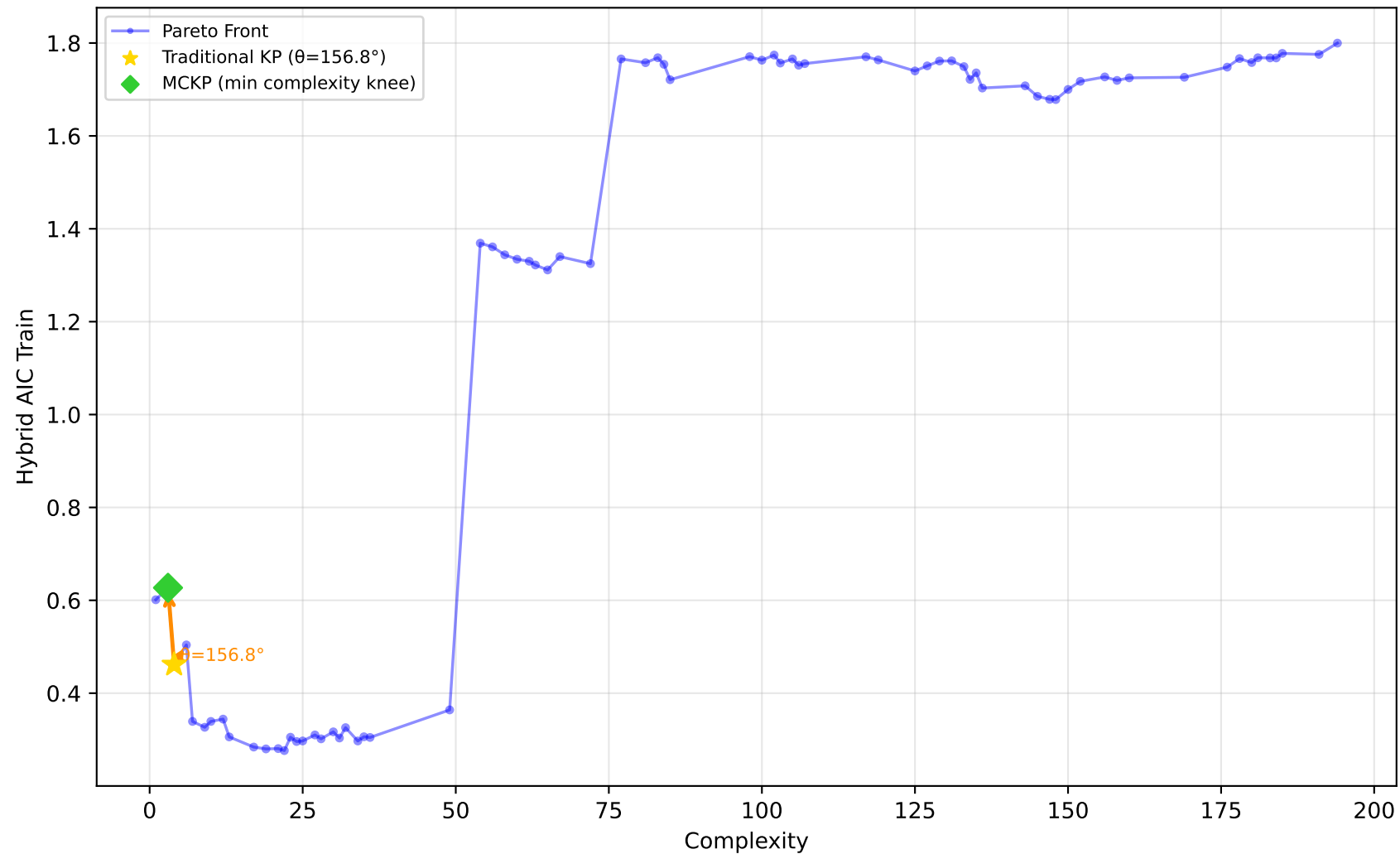
228_elusage - Run 7 - SVP - Hybrid AIC Train \lambda_1=0.60, \lambda_2=0.60, \lambda_3=1.00 | Difficulty: 1.00 | Method: hmr
