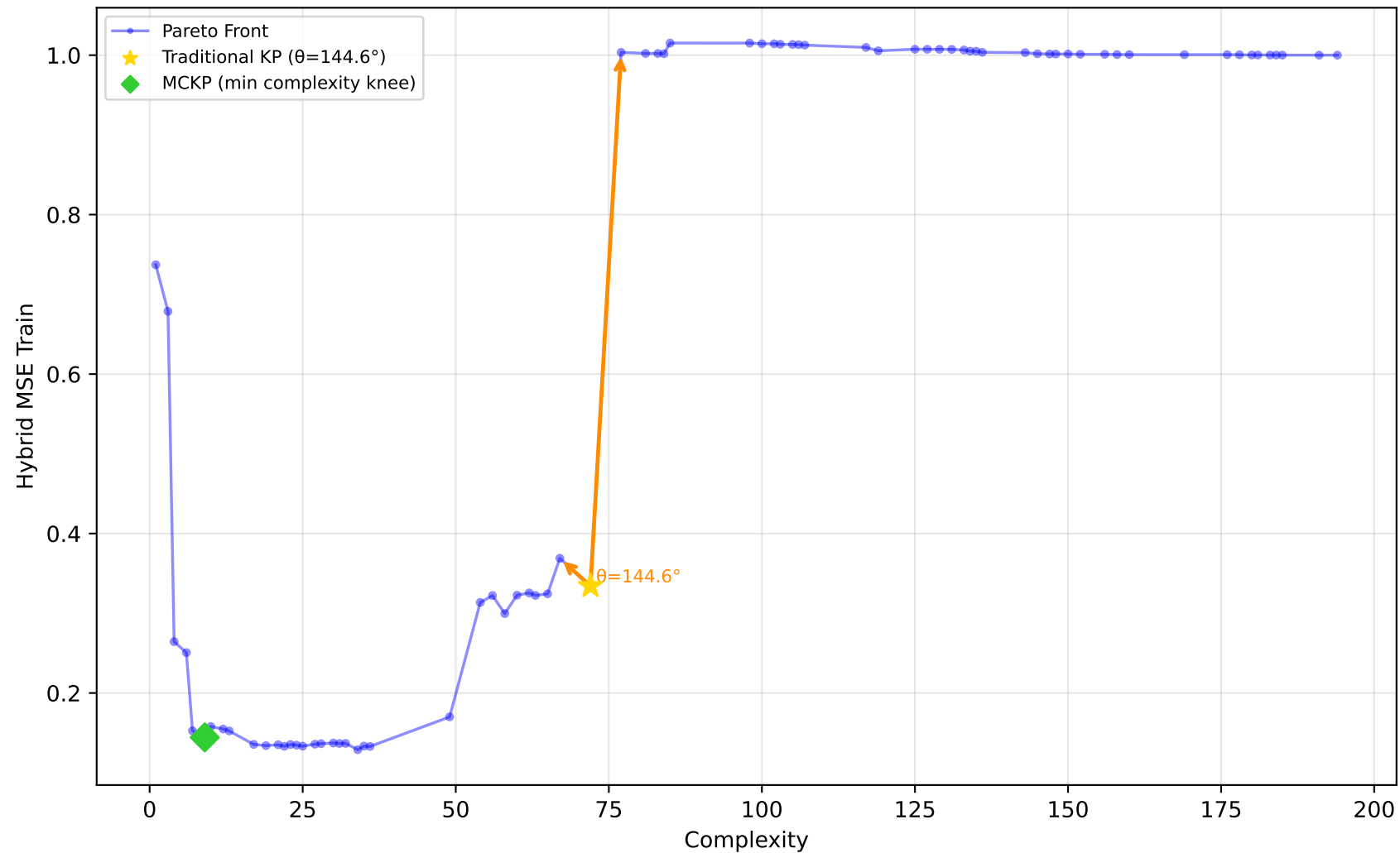
228_elusage - Run 7 - SVP - Hybrid MSE Train \lambda_1=0.00, \lambda_2=1.00, \lambda_3=0.00 | Difficulty: 1.00 | Method: hmr
