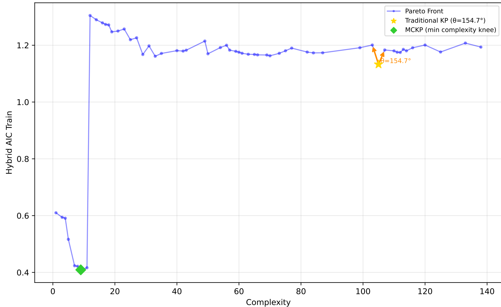
228_elusage - Run 8 - MVP - Hybrid AIC Train \lambda_1=0.00, \lambda_2=0.00, \lambda_3=1.00 | Difficulty: 0.92 | Method: hmr
