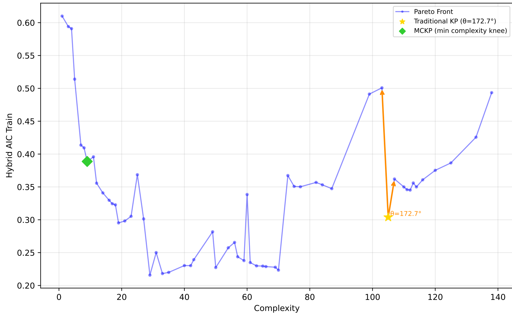
228_elusage - Run 8 - MVP - Hybrid AIC Train \lambda_1=0.00, \lambda_2=0.30, \lambda_3=0.00 | Difficulty: 0.92 | Method: hmr
