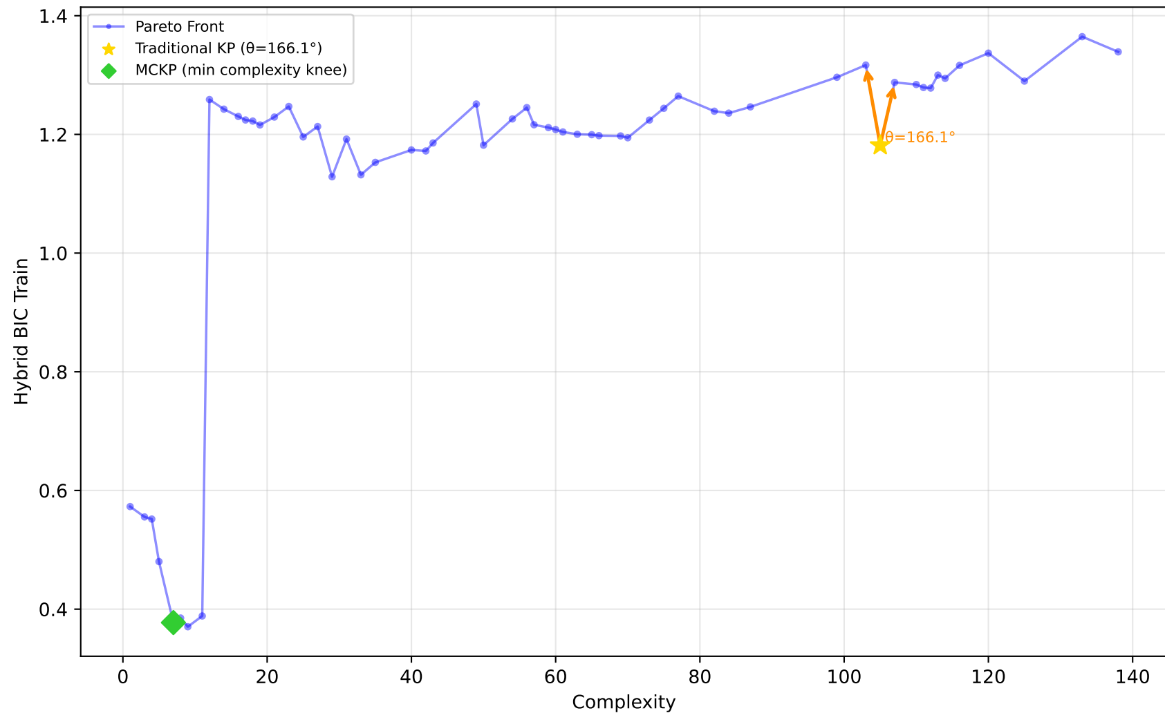
228_elusage - Run 8 - MVP - Hybrid BIC Train \lambda_1=0.00, \lambda_2=0.00, \lambda_3=1.00 | Difficulty: 0.92 | Method: hmr
