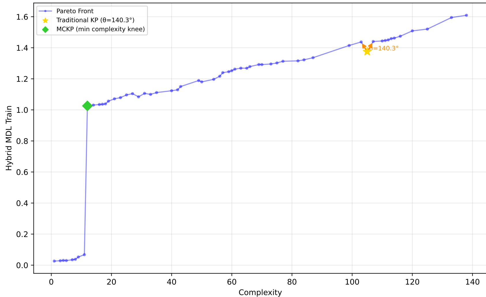
228_elusage - Run 8 - MVP - Hybrid MDL Train \lambda_1=0.00, \lambda_2=0.00, \lambda_3=1.00 | Difficulty: 0.92 | Method: hmr
