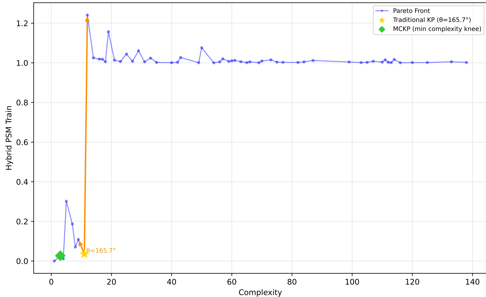
228_elusage - Run 8 - MVP - Hybrid PSM Train \lambda_1=0.00, \lambda_2=0.00, \lambda_3=1.00 | Difficulty: 0.92 | Method: hmr
