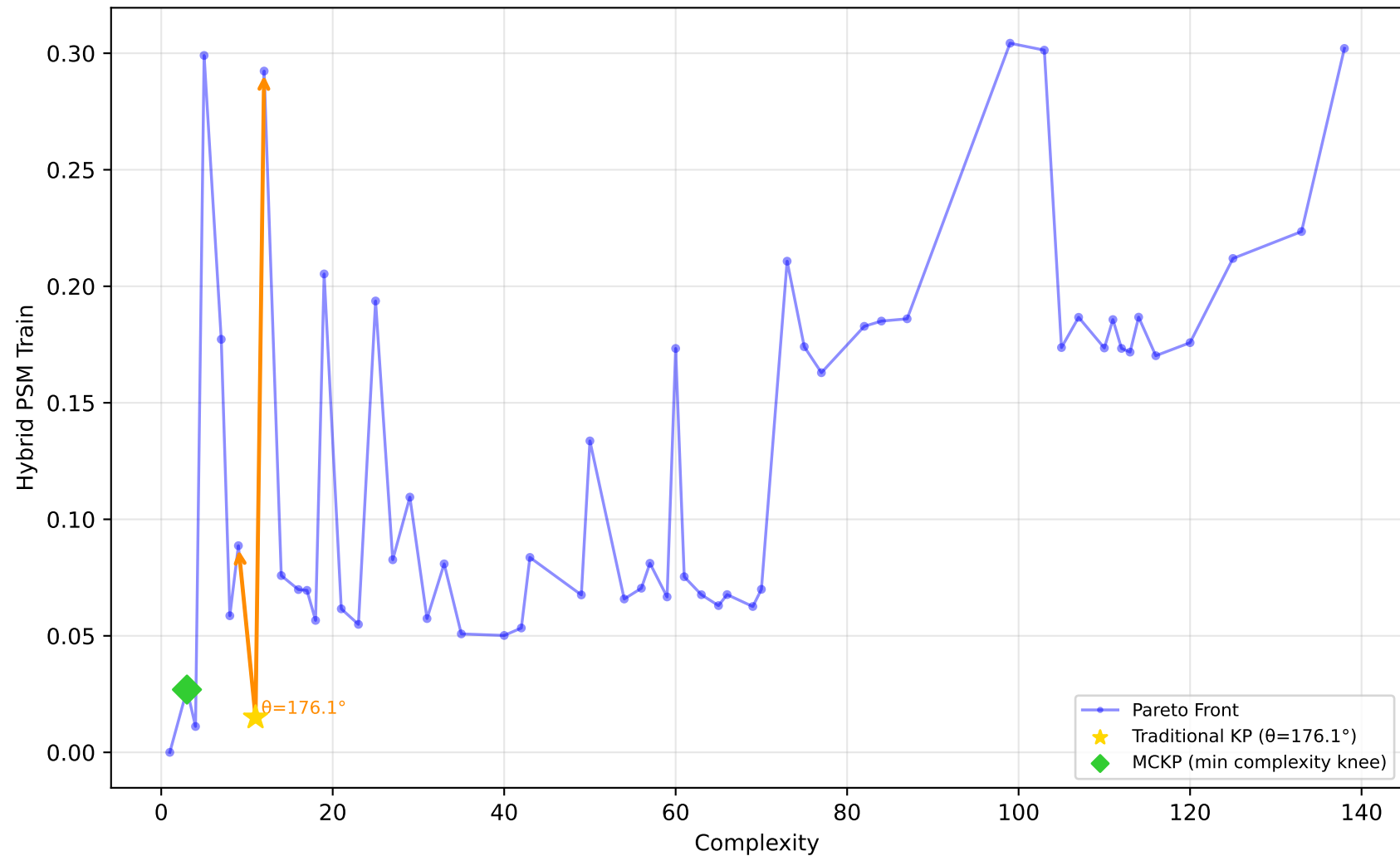
228_elusage - Run 8 - MVP - Hybrid PSM Train \lambda_1=0.00, \lambda_2=0.30, \lambda_3=0.00 | Difficulty: 0.92 | Method: hmr
