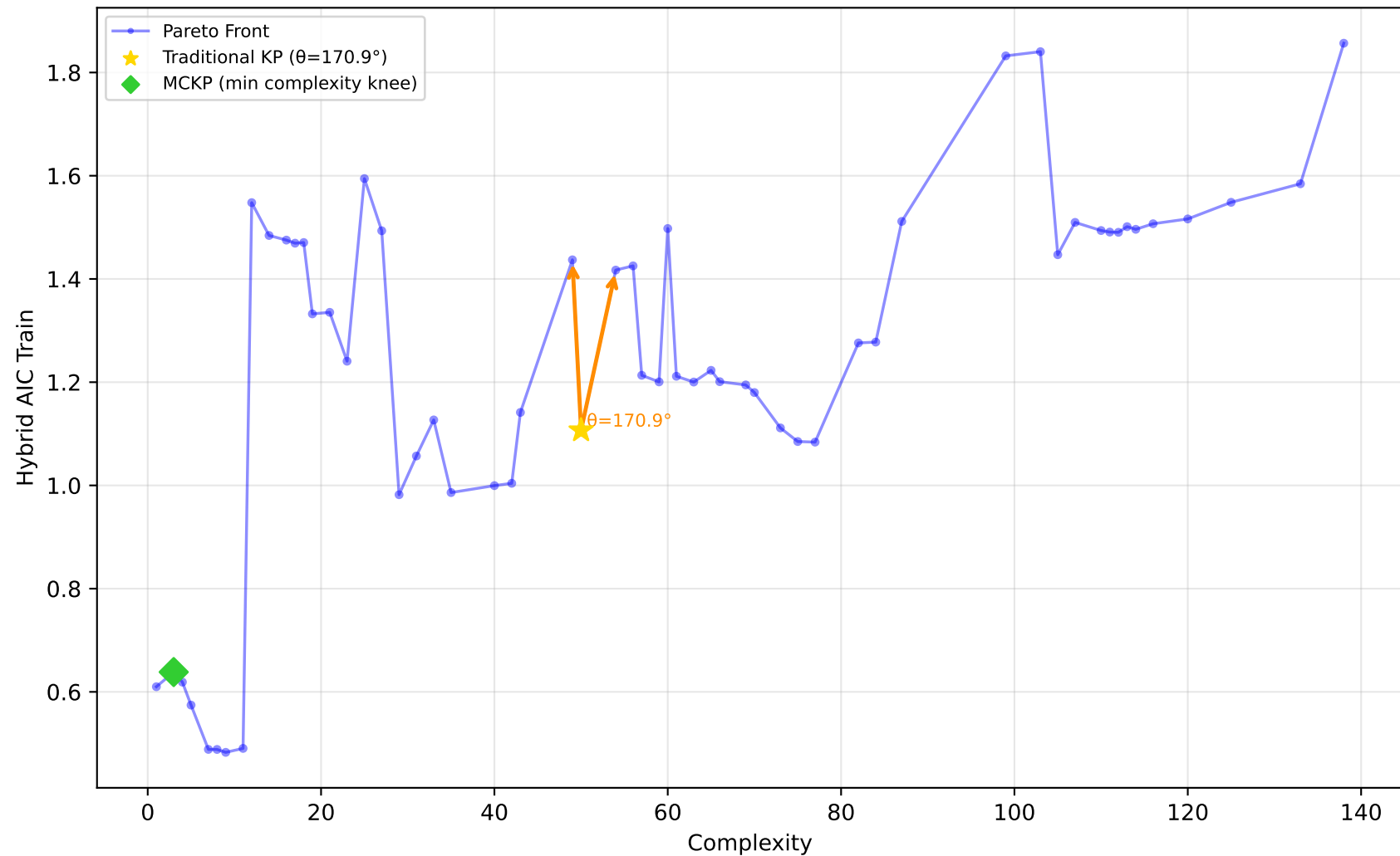
228_elusage - Run 8 - SVP - Hybrid AIC Train \lambda_1=0.60, \lambda_2=0.60, \lambda_3=1.00 | Difficulty: 0.92 | Method: hmr
