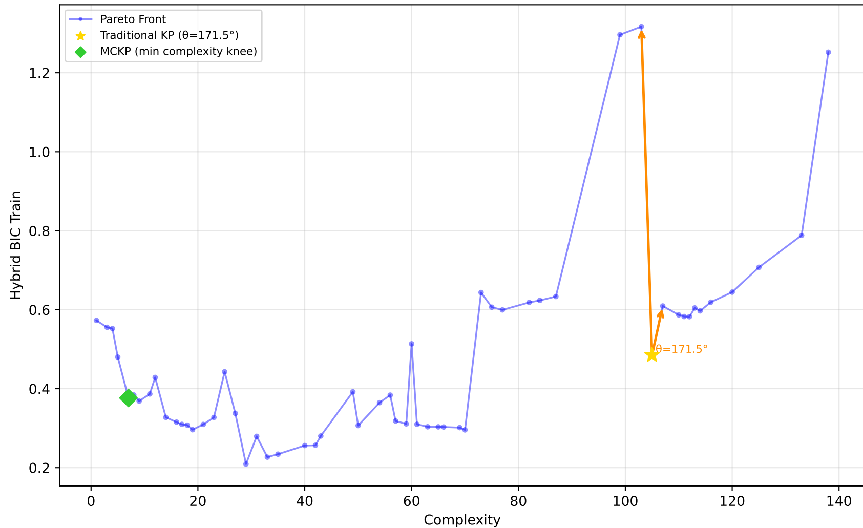
228_elusage - Run 8 - SVP - Hybrid BIC Train \lambda_1=0.00, \lambda_2=1.00, \lambda_3=0.00 | Difficulty: 0.92 | Method: hmr
