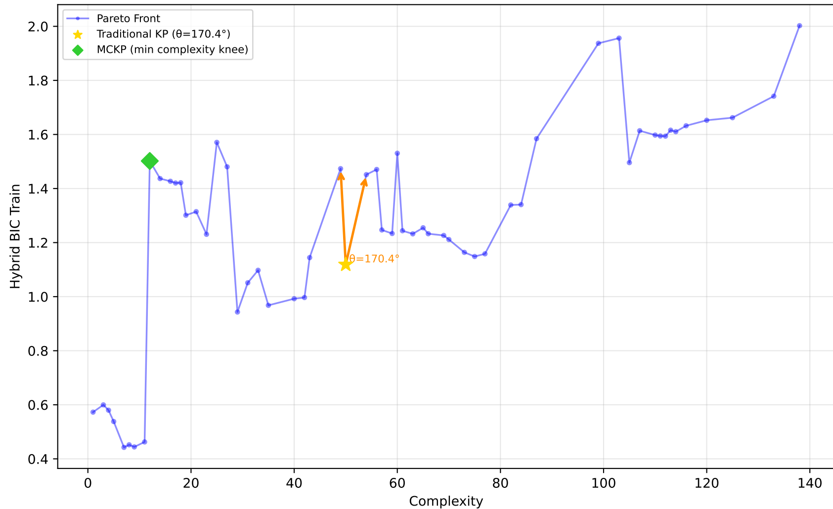
228_elusage - Run 8 - SVP - Hybrid BIC Train \lambda_1=0.60, \lambda_2=0.60, \lambda_3=1.00 | Difficulty: 0.92 | Method: hmr
