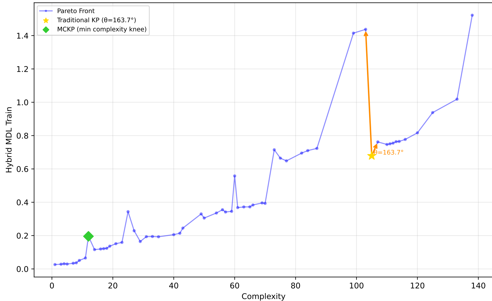
228_elusage - Run 8 - SVP - Hybrid MDL Train \lambda_1=0.00, \lambda_2=1.00, \lambda_3=0.00 | Difficulty: 0.92 | Method: hmr
