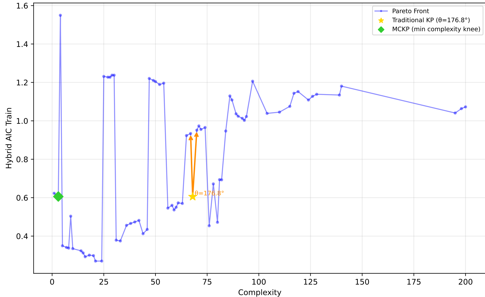
228_elusage - Run 9 - MVP - Hybrid AIC Train \lambda_1=0.00, \lambda_2=0.00, \lambda_3=1.00 | Difficulty: 0.72 | Method: hmr
