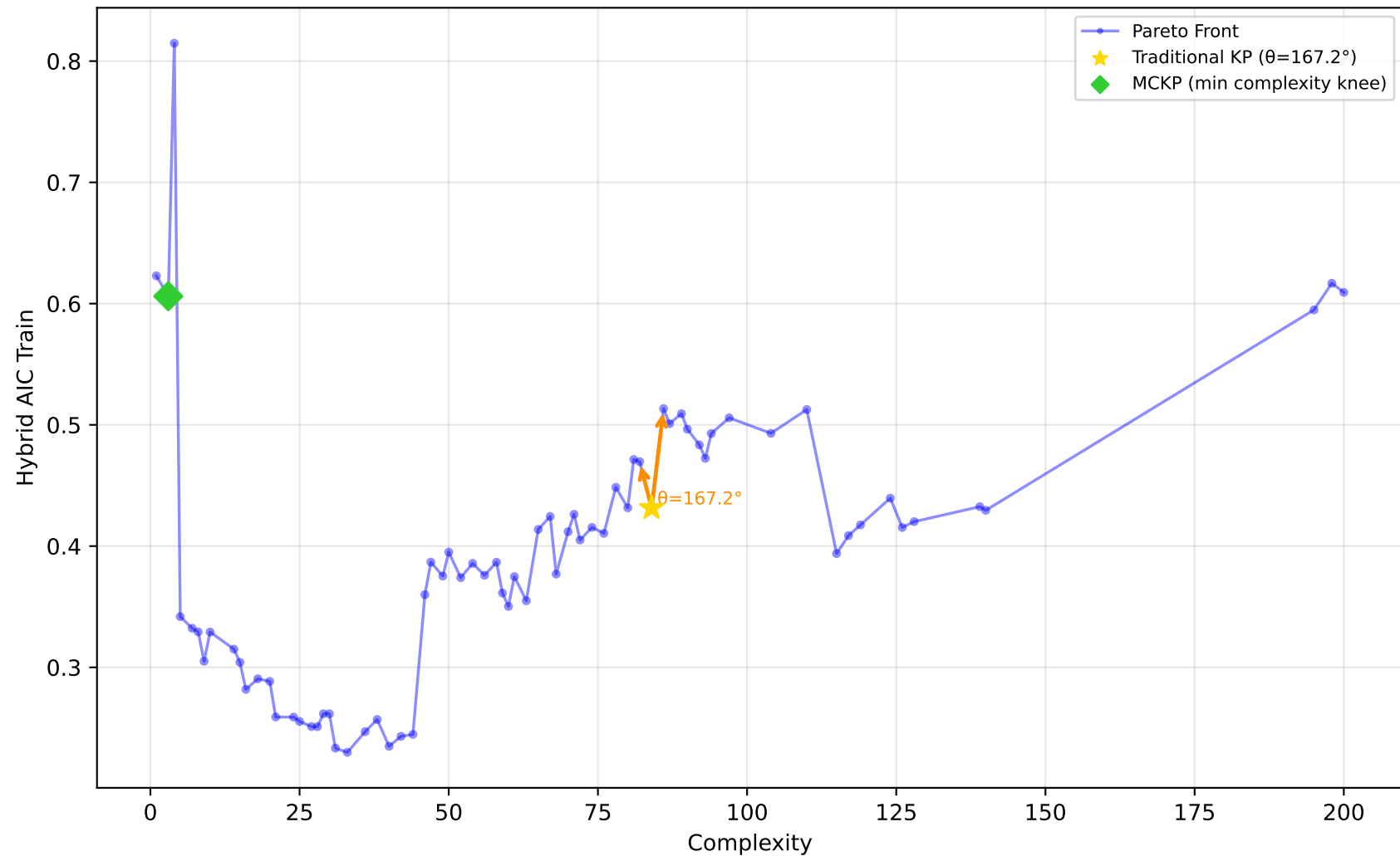
228_elusage - Run 9 - MVP - Hybrid AIC Train \lambda_1=0.00, \lambda_2=0.30, \lambda_3=0.00 | Difficulty: 0.72 | Method: hmr
