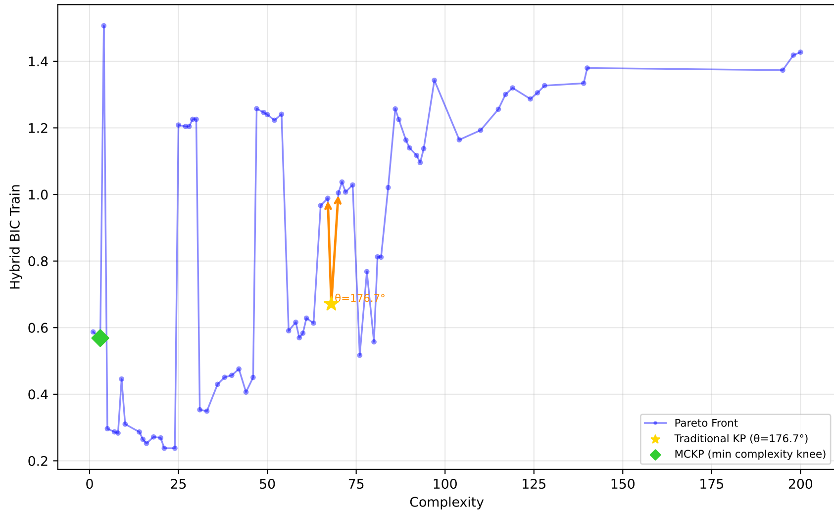
228_elusage - Run 9 - MVP - Hybrid BIC Train \lambda_1=0.00, \lambda_2=0.00, \lambda_3=1.00 | Difficulty: 0.72 | Method: hmr
