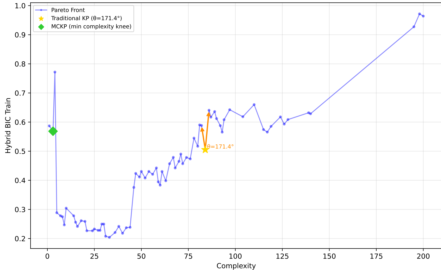
228_elusage - Run 9 - MVP - Hybrid BIC Train \lambda_1=0.00, \lambda_2=0.30, \lambda_3=0.00 | Difficulty: 0.72 | Method: hmr
