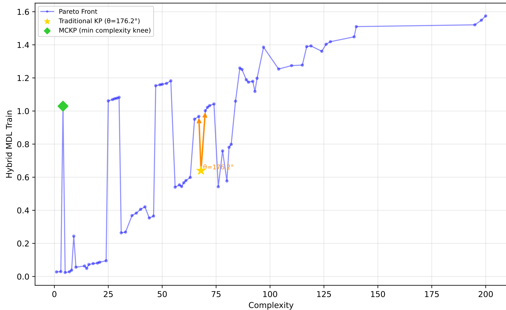
228_elusage - Run 9 - MVP - Hybrid MDL Train \lambda_1=0.00, \lambda_2=0.00, \lambda_3=1.00 | Difficulty: 0.72 | Method: hmr
