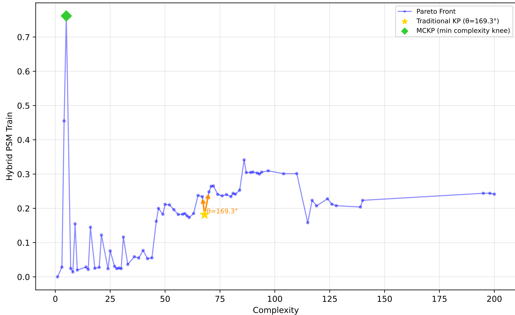
228_elusage - Run 9 - MVP - Hybrid PSM Train \lambda_1=0.00, \lambda_2=0.30, \lambda_3=0.00 | Difficulty: 0.72 | Method: hmr
