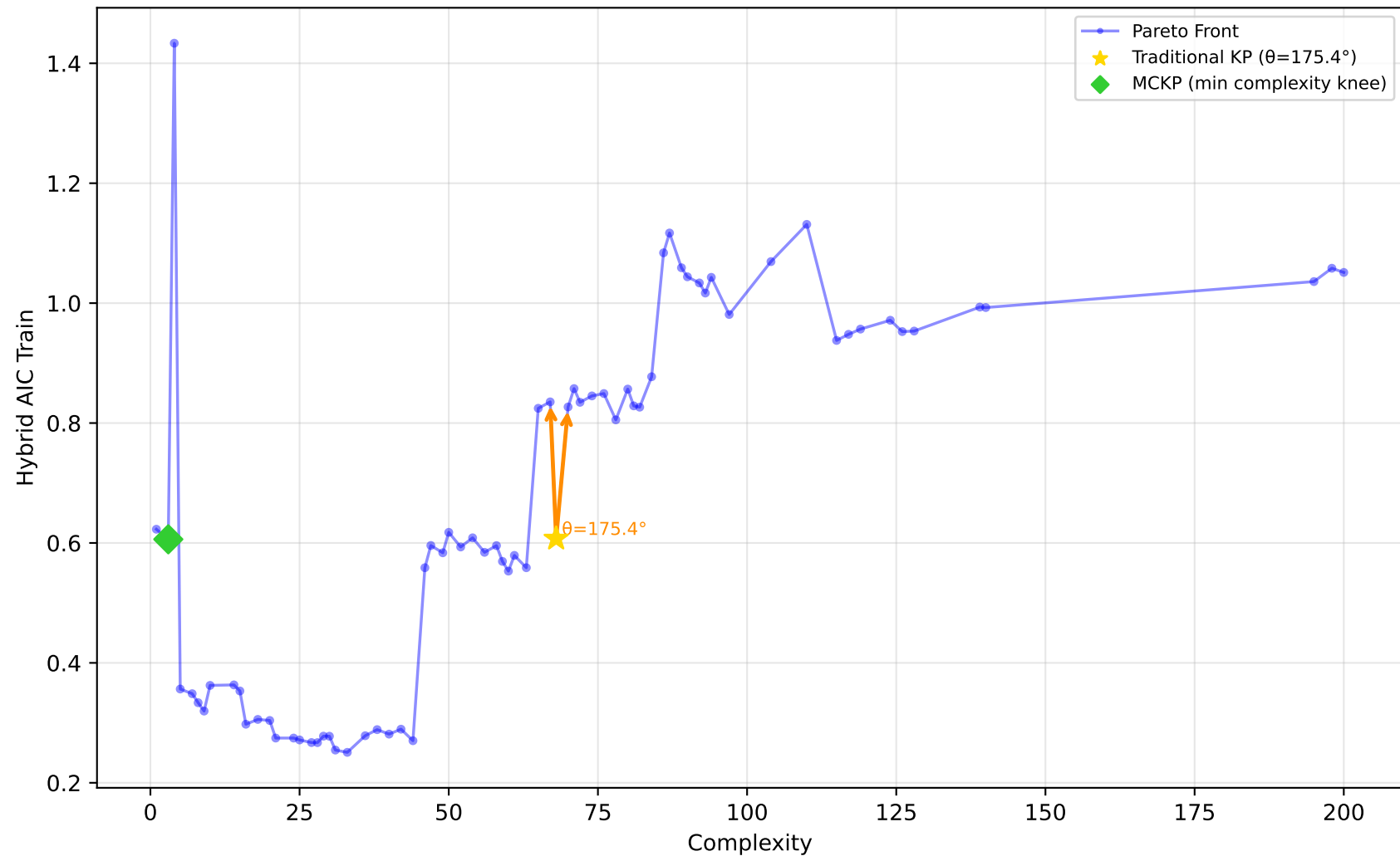
228_elusage - Run 9 - SVP - Hybrid AIC Train \lambda_1=0.00, \lambda_2=1.00, \lambda_3=0.00 | Difficulty: 0.72 | Method: hmr
