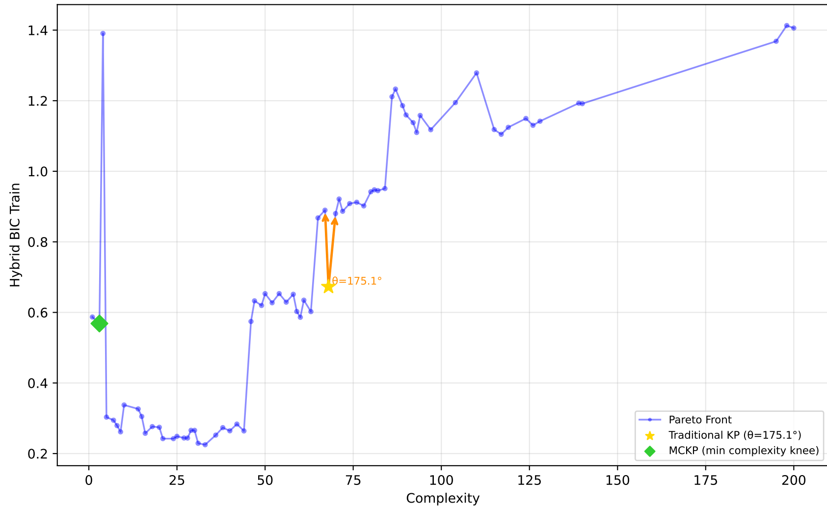
228_elusage - Run 9 - SVP - Hybrid BIC Train \lambda_1=0.00, \lambda_2=1.00, \lambda_3=0.00 | Difficulty: 0.72 | Method: hmr
