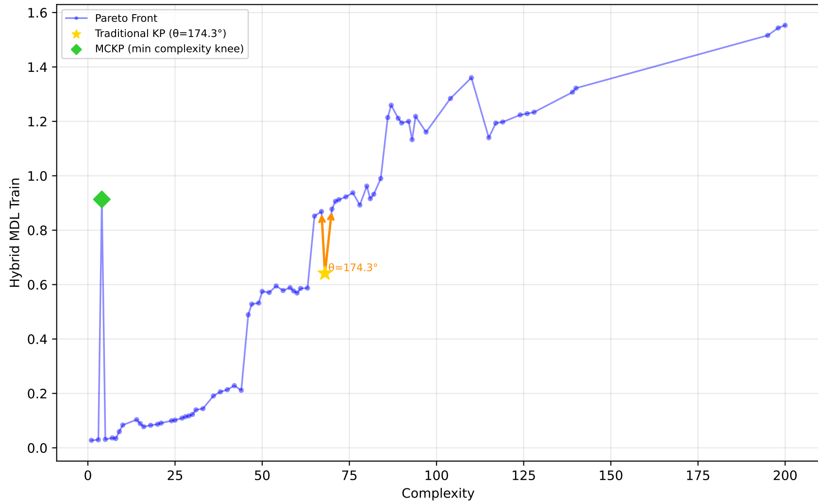
228_elusage - Run 9 - SVP - Hybrid MDL Train \lambda_1=0.00 , \lambda_2=1.00 , \lambda_3=0.00 | Difficulty: 0.72 | Method: hmr
