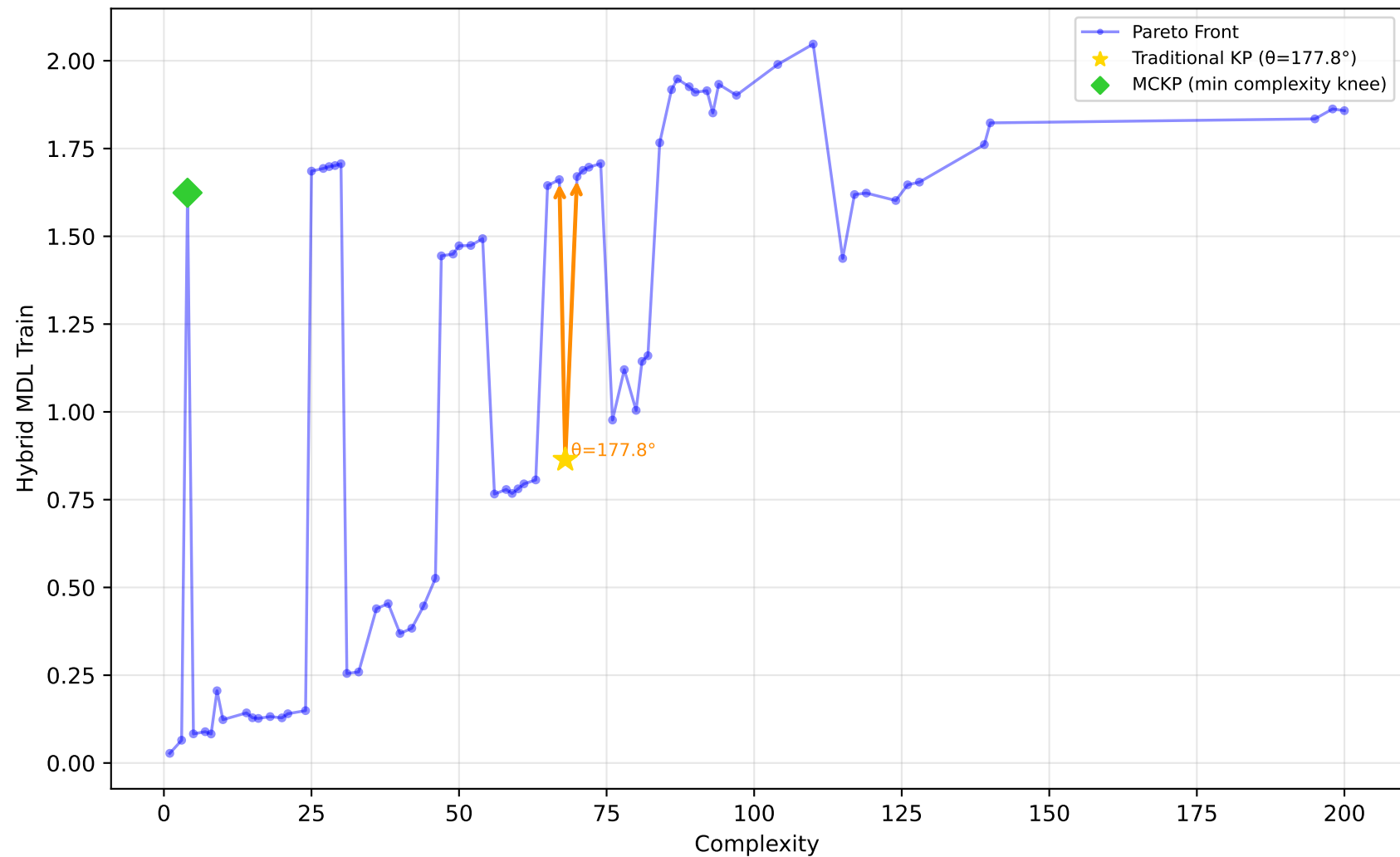
228_elusage - Run 9 - SVP - Hybrid MDL Train \lambda_1=0.60 , \lambda_2=0.60 , \lambda_3=1.00 | Difficulty: 0.72 | Method: hmr
