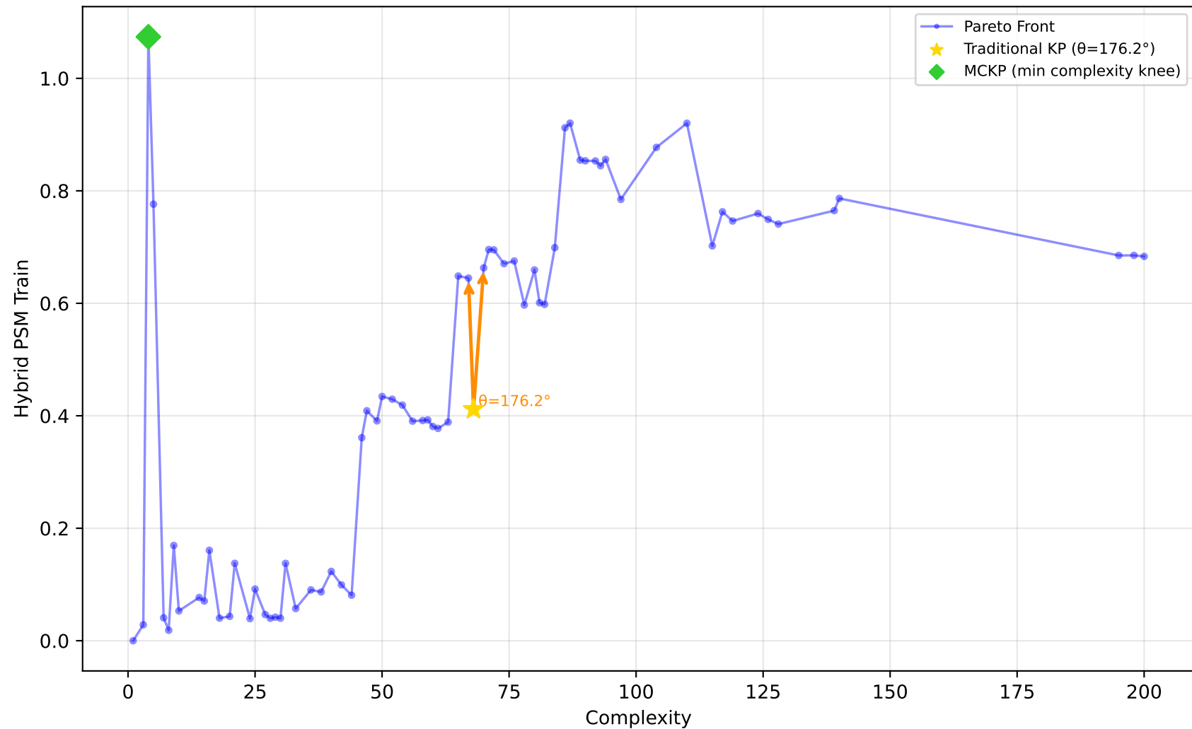
228_elusage - Run 9 - SVP - Hybrid PSM Train \lambda_1=0.00, \lambda_2=1.00, \lambda_3=0.00 | Difficulty: 0.72 | Method: hmr
