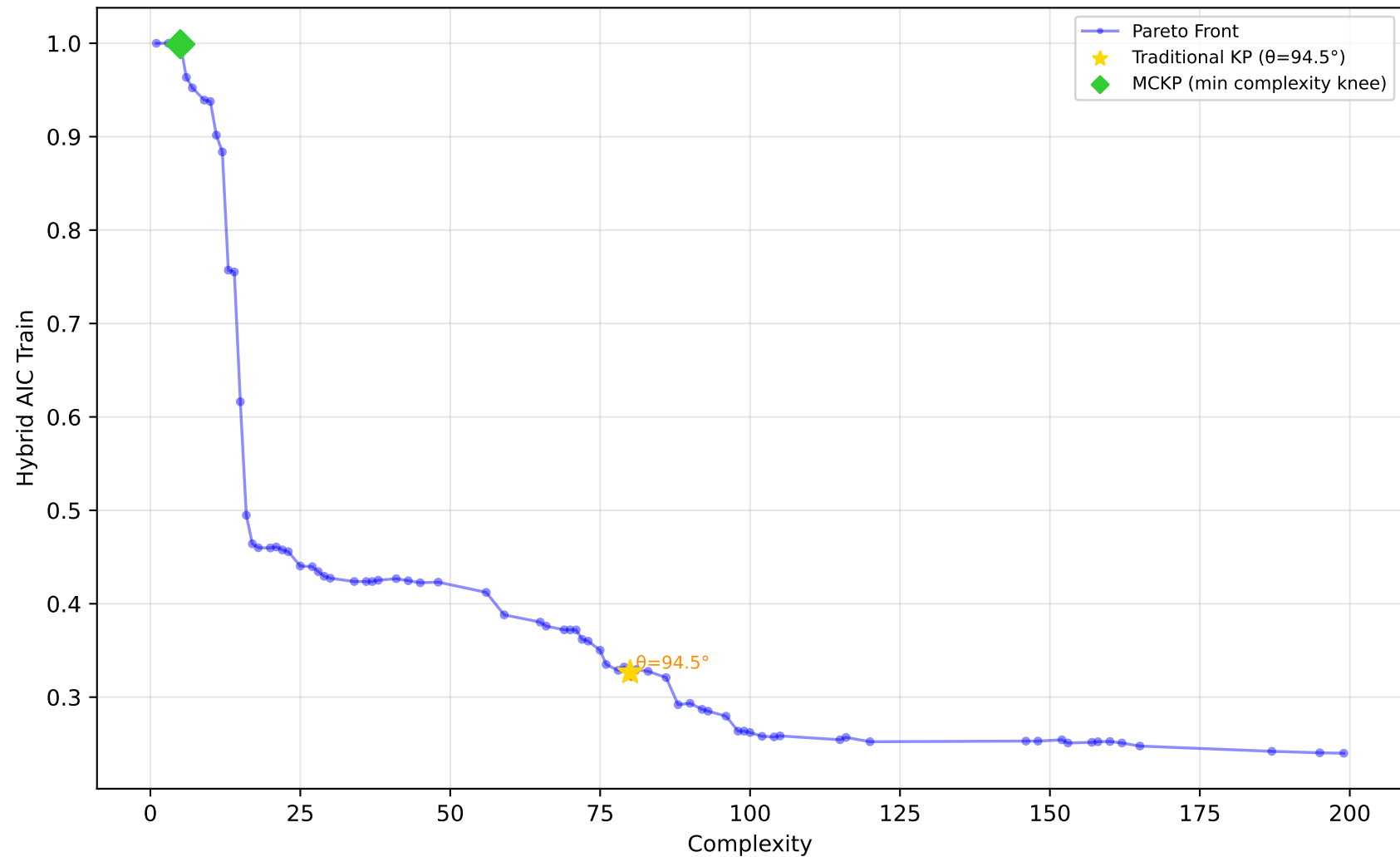
556_analcatdata_apnea2 - Run 10 - MVP - Hybrid AIC Train \lambda_1=0.00, \lambda_2=0.00, \lambda_3=0.00 | Difficulty: 1.00 | Method: hmr
