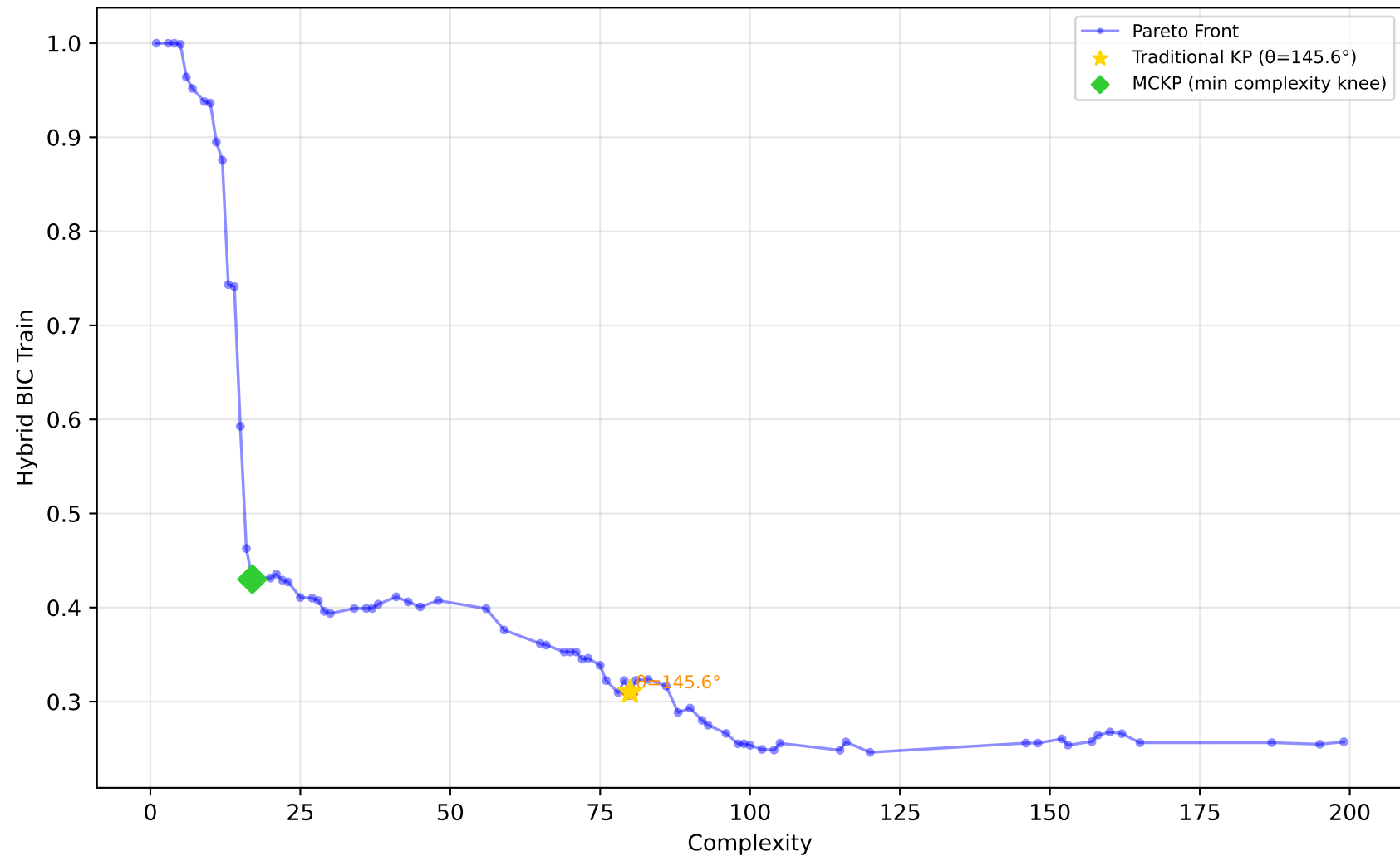
556_analcatdata_apnea2 - Run 10 - SVP - Hybrid BIC Train \lambda_1=0.00, \lambda_2=0.00, \lambda_3=0.00 | Difficulty: 1.00 | Method: hmr
