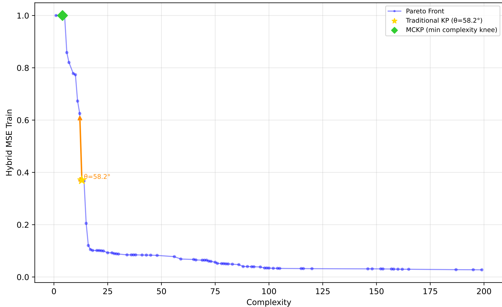
556_analcatdata_apnea2 - Run 10 - SVP - Hybrid MSE Train \lambda_1=0.00, \lambda_2=0.00, \lambda_3=0.00 | Difficulty: 1.00 | Method: hmr
