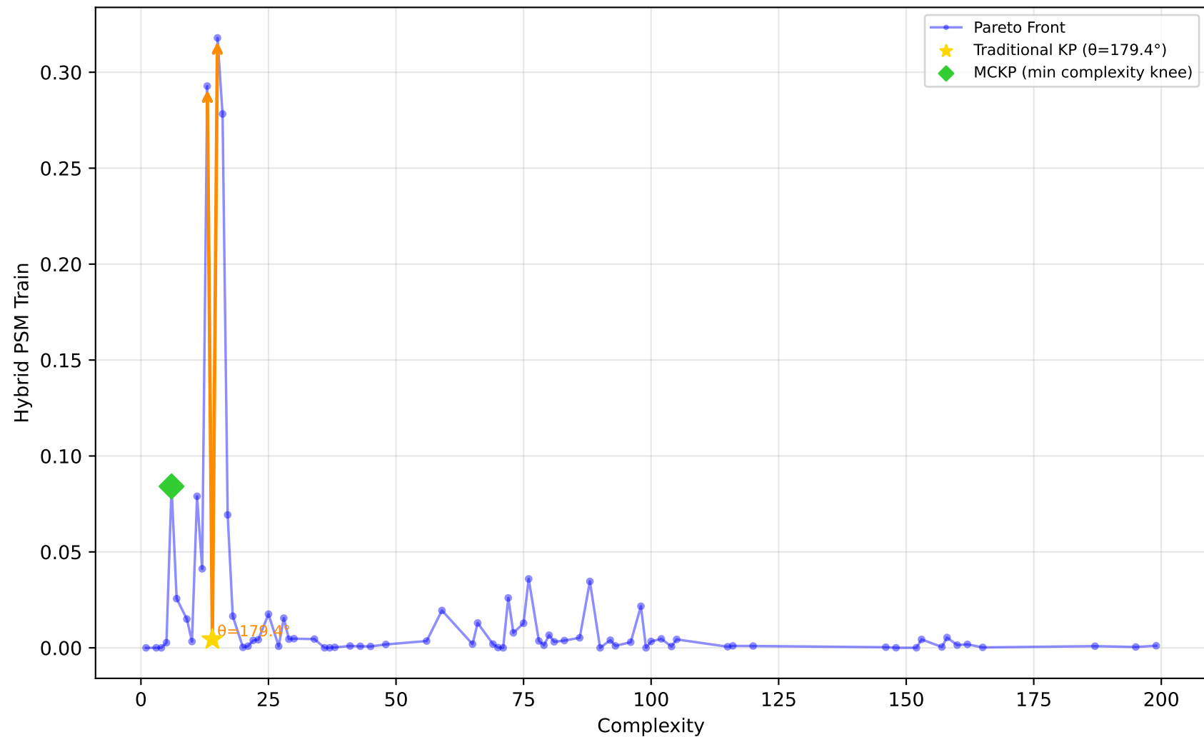
556_analcatdata_apnea2 - Run 10 - SVP - Hybrid PSM Train \lambda_1=0.00 , \lambda_2=0.00 , \lambda_3=0.00 | Difficulty: 1.00 | Method: hmr
