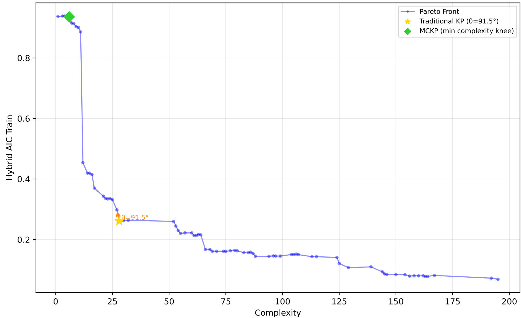
556_analcatdata_apnea2 - Run 11 - MVP - Hybrid AIC Train \lambda_1=0.00, \lambda_2=0.00, \lambda_3=0.00 | Difficulty: 1.00 | Method: hmr
