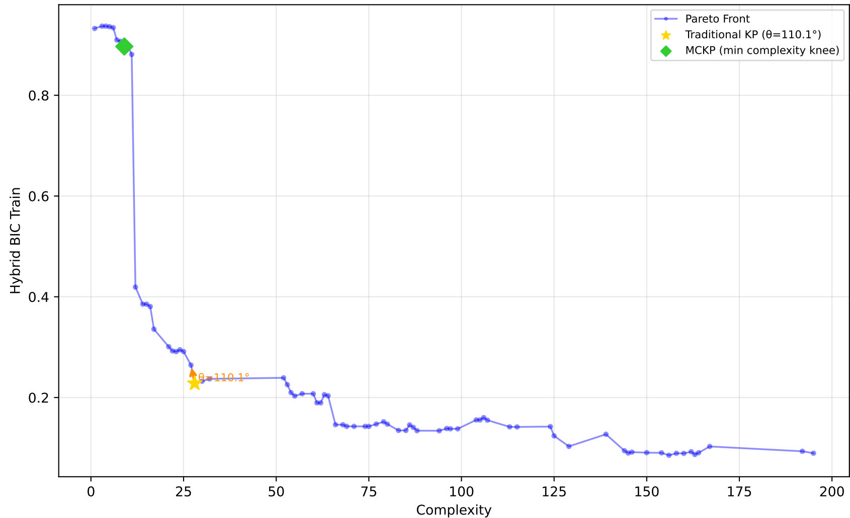
556_analcatdata_apnea2 - Run 11 - MVP - Hybrid BIC Train \lambda_1=0.00, \lambda_2=0.00, \lambda_3=0.00 | Difficulty: 1.00 | Method: hmr
