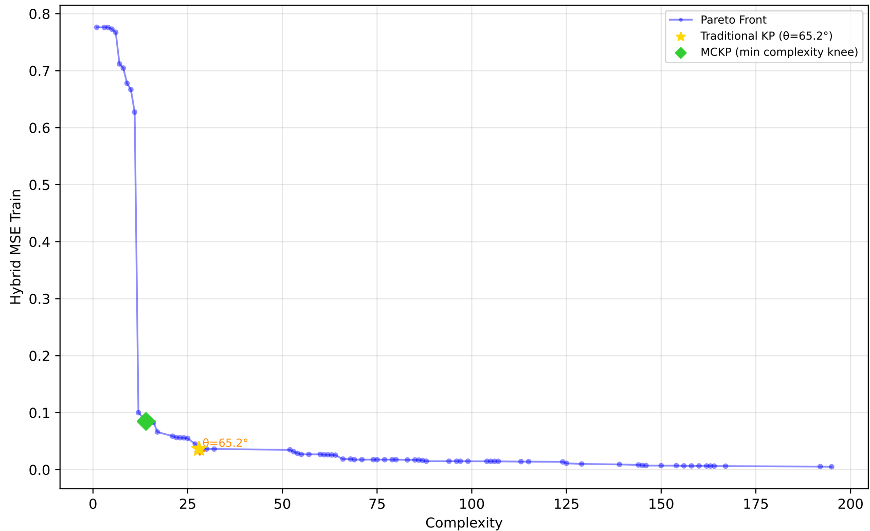
556_analcatdata_apnea2 - Run 11 - SVP - Hybrid MSE Train \lambda_1=0.00, \lambda_2=0.00, \lambda_3=0.00 | Difficulty: 1.00 | Method: hmr
