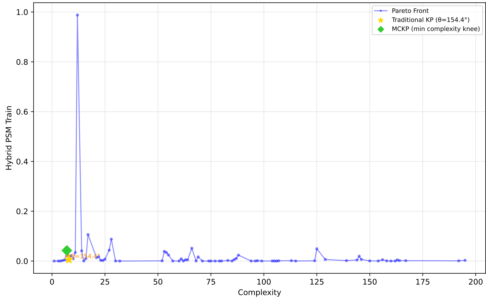
556_analcatdata_apnea2 - Run 11 - SVP - Hybrid PSM Train \lambda_1=0.00 , \lambda_2=0.00 , \lambda_3=0.00 | Difficulty: 1.00 | Method: hmr
