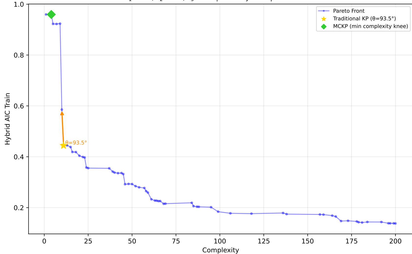
556_analcatdata_apnea2 - Run 12 - MVP - Hybrid AIC Train \lambda_1=0.00, \lambda_2=0.00, \lambda_3=0.00 | Difficulty: 0.83 | Method: hmr
