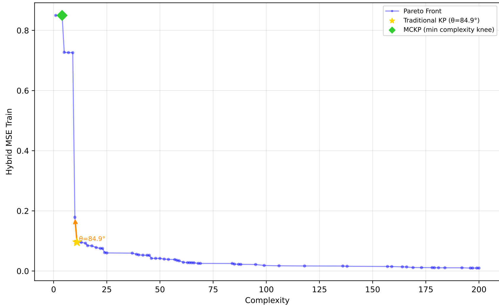
556_analcatdata_apnea2 - Run 12 - MVP - Hybrid MSE Train \lambda_1=0.00, \lambda_2=0.00, \lambda_3=0.00 | Difficulty: 0.83 | Method: hmr
