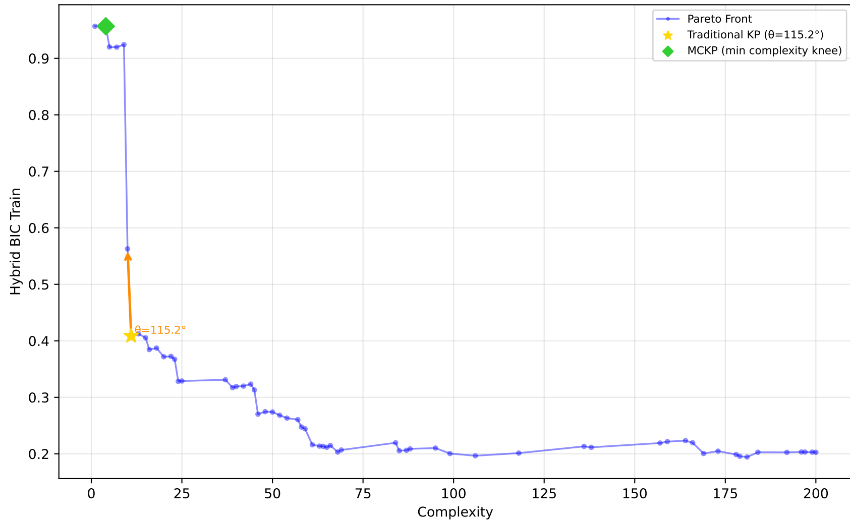
556_analcatdata_apnea2 - Run 12 - SVP - Hybrid BIC Train \lambda_1=0.00, \lambda_2=0.00, \lambda_3=0.00 | Difficulty: 0.83 | Method: hmr
