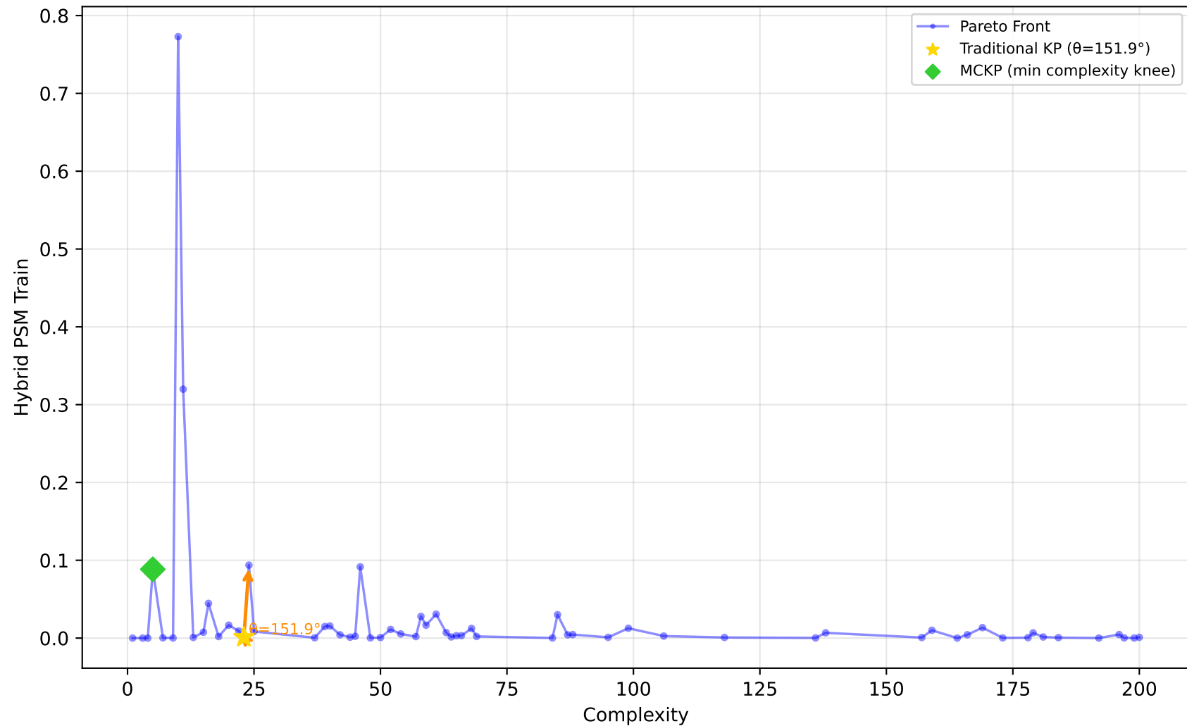
556_analcatdata_apnea2 - Run 12 - SVP - Hybrid PSM Train \lambda_1=0.00, \lambda_2=0.00, \lambda_3=0.00 | Difficulty: 0.83 | Method: hmr
