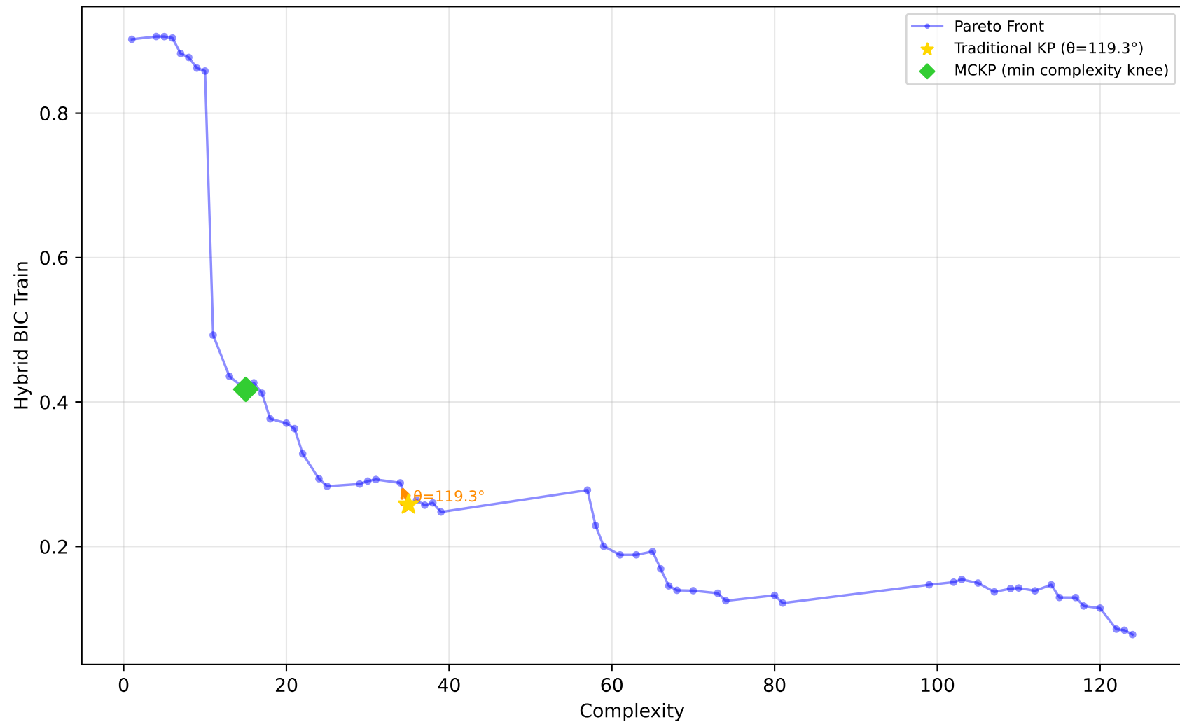
556_analcatdata_apnea2 - Run 13 - MVP - Hybrid BIC Train \lambda_1=0.00, \lambda_2=0.00, \lambda_3=0.00 | Difficulty: 1.00 | Method: hmr
