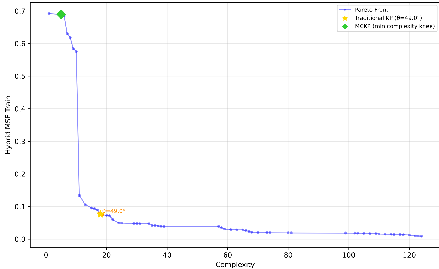
556_analcatdata_apnea2 - Run 13 - MVP - Hybrid MSE Train \lambda_1=0.00, \lambda_2=0.00, \lambda_3=0.00 | Difficulty: 1.00 | Method: hmr
