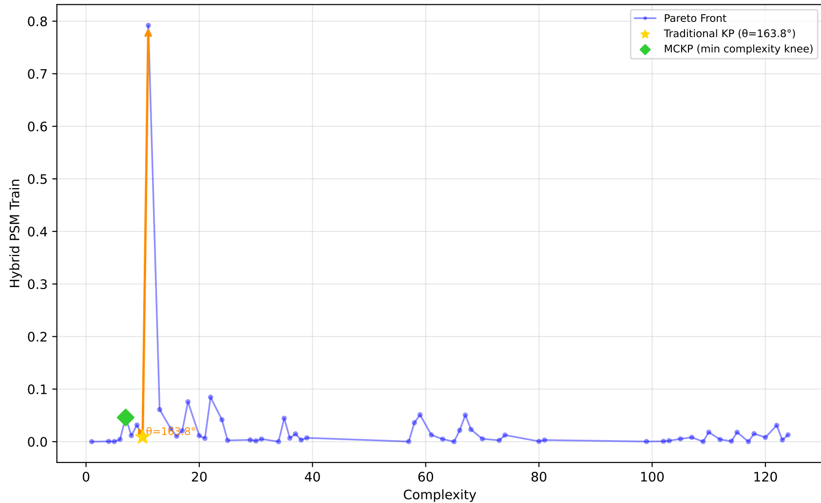
556_analcatdata_apnea2 - Run 13 - SVP - Hybrid PSM Train \lambda_1=0.00, \lambda_2=0.00, \lambda_3=0.00 | Difficulty: 1.00 | Method: hmr
