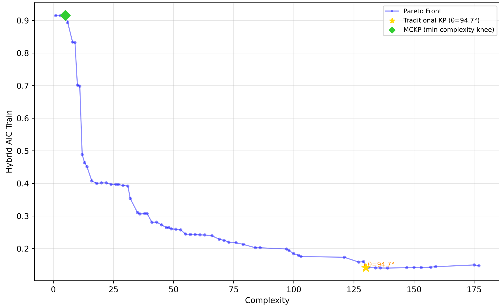
556_analcatdata_apnea2 - Run 14 - MVP - Hybrid AIC Train \lambda_1=0.00, \lambda_2=0.00, \lambda_3=0.00 | Difficulty: 1.00 | Method: hmr
