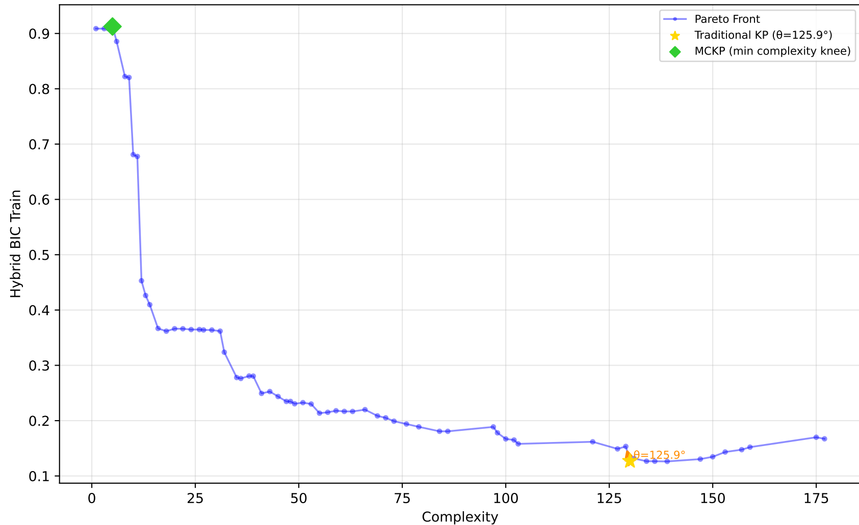
556_analcatdata_apnea2 - Run 14 - SVP - Hybrid BIC Train \lambda_1=0.00, \lambda_2=0.00, \lambda_3=0.00 | Difficulty: 1.00 | Method: hmr
