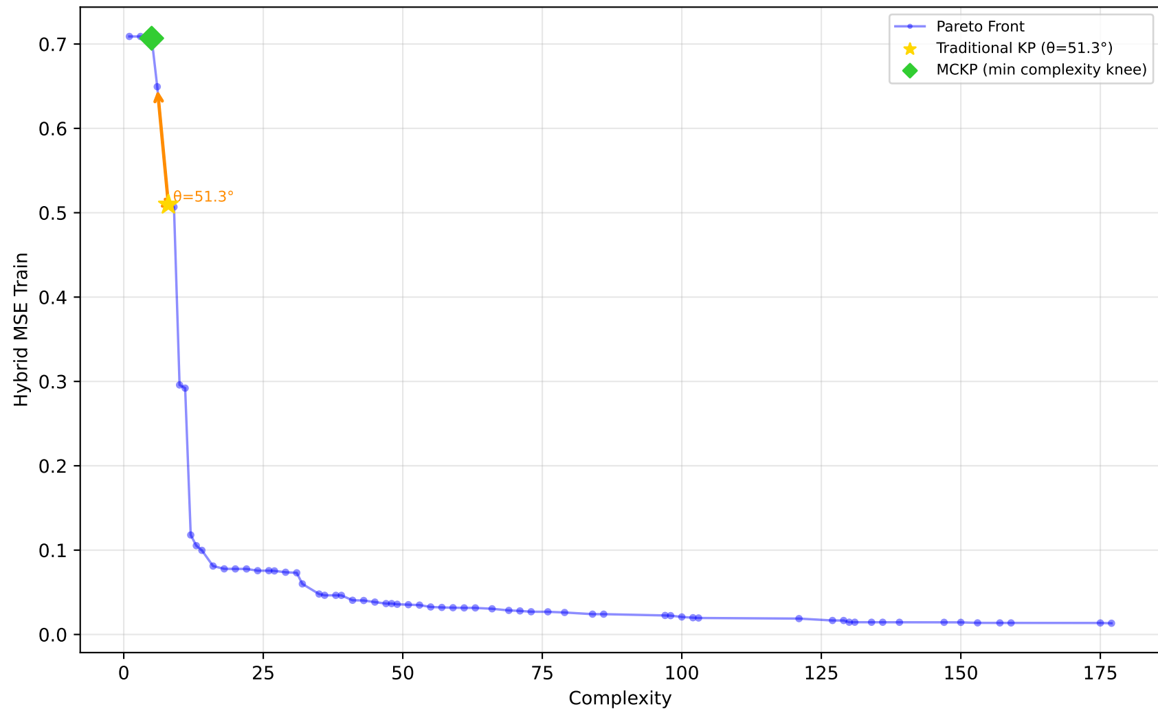
556_analcatdata_apnea2 - Run 14 - SVP - Hybrid MSE Train \lambda_1=0.00, \lambda_2=0.00, \lambda_3=0.00 | Difficulty: 1.00 | Method: hmr
