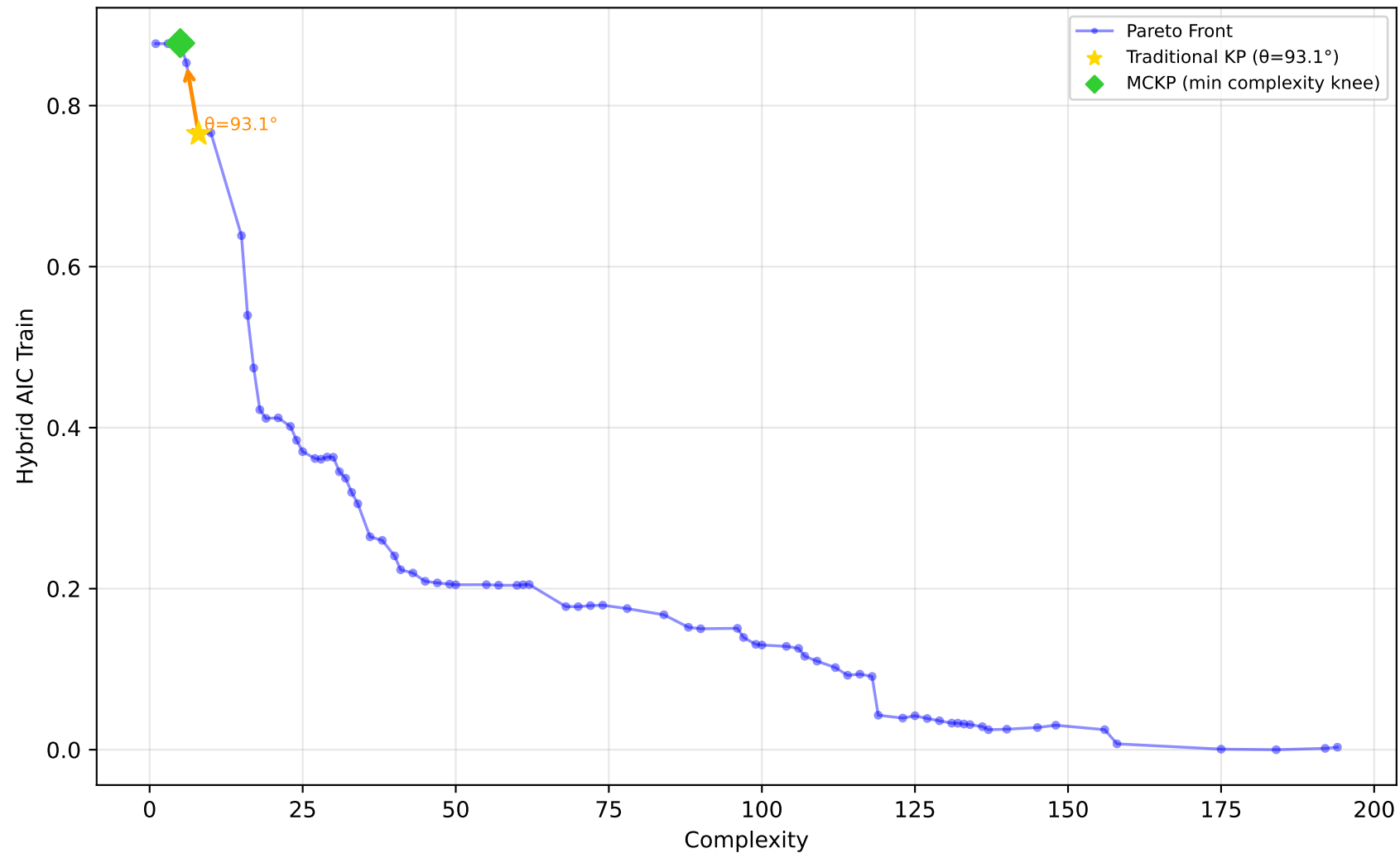
556_analcatdata_apnea2 - Run 15 - MVP - Hybrid AIC Train \lambda_1=0.00, \lambda_2=0.00, \lambda_3=0.00 | Difficulty: 1.00 | Method: hmr
