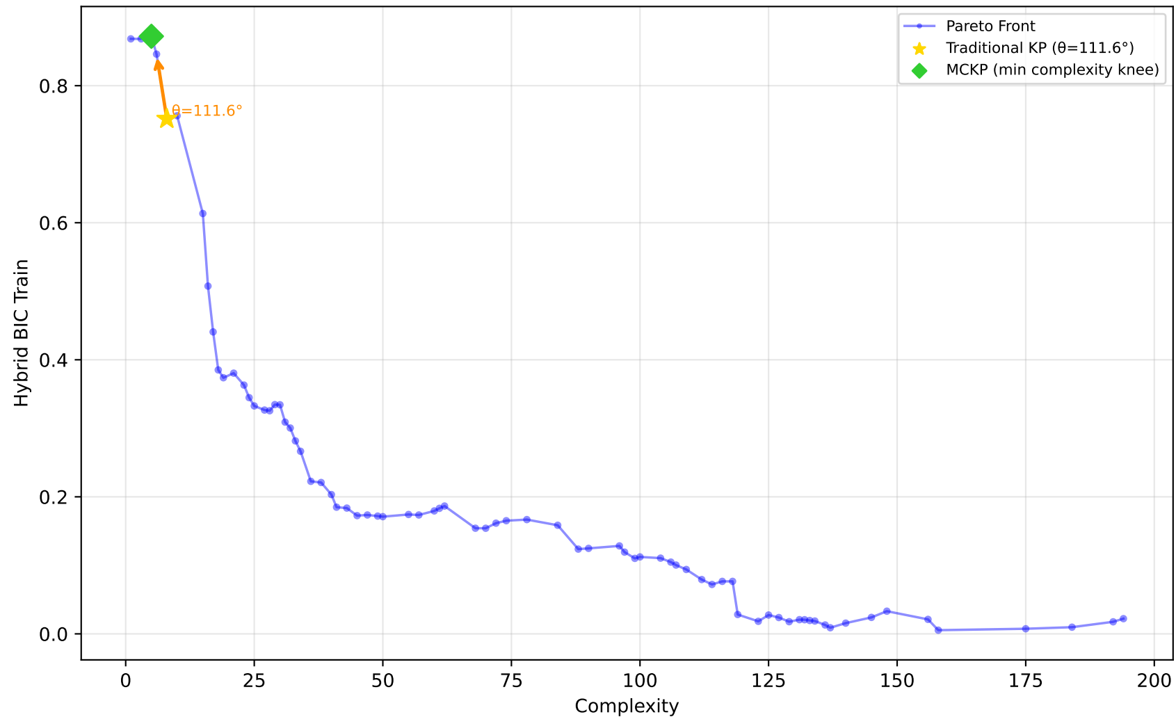
556_analcatdata_apnea2 - Run 15 - MVP - Hybrid BIC Train \lambda_1=0.00, \lambda_2=0.00, \lambda_3=0.00 | Difficulty: 1.00 | Method: hmr
